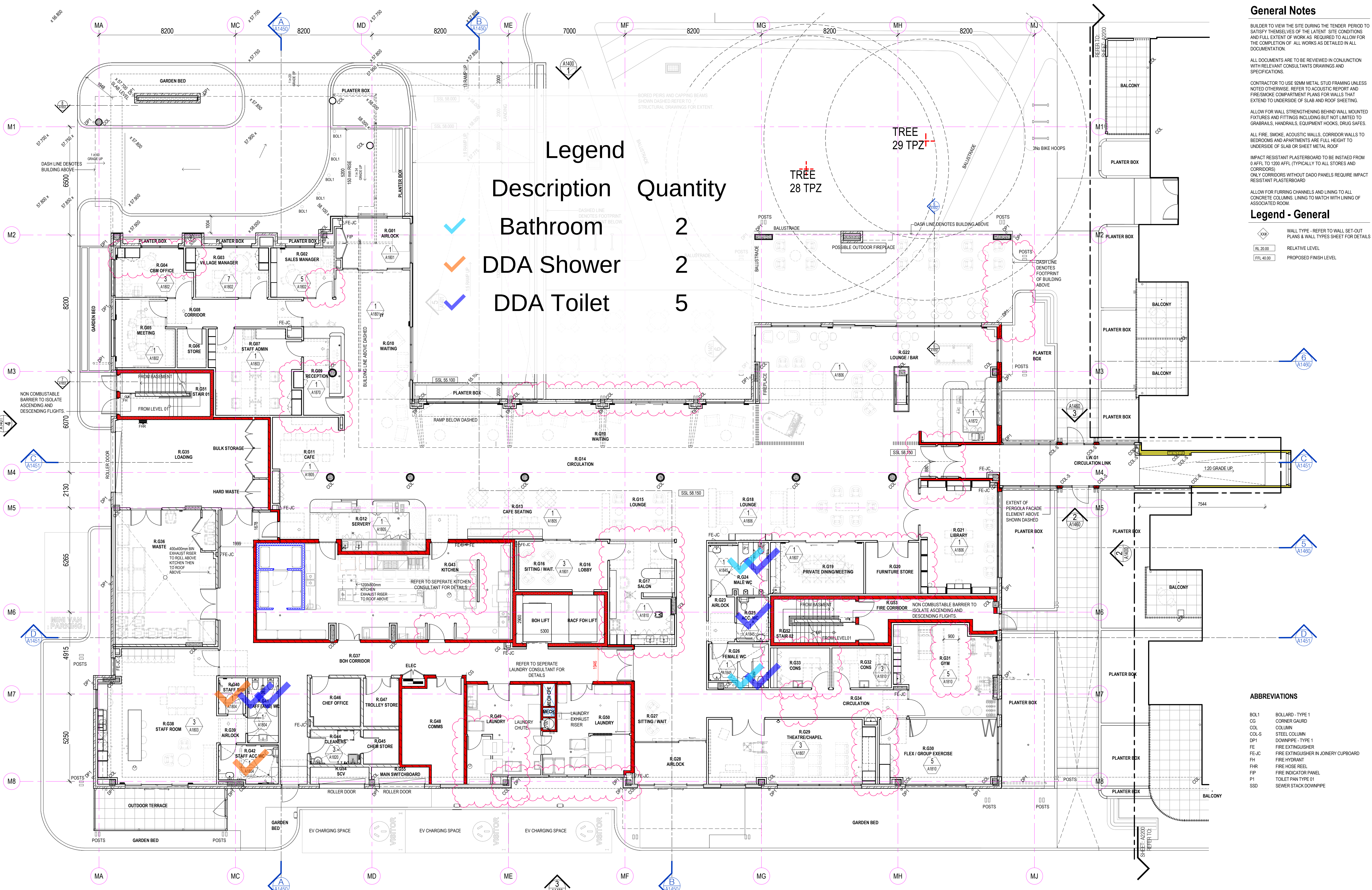
3 GROUND FLOOR PLAN - RACF Scale 1:100
